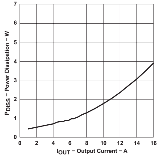
Figure 17. Power Dissipation vs. Load
