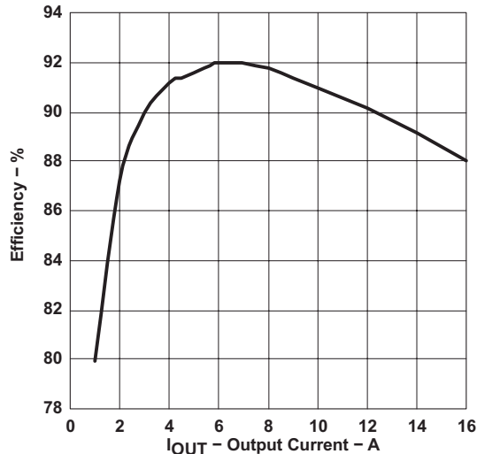
Figure 16. Efficiency vs. Load
