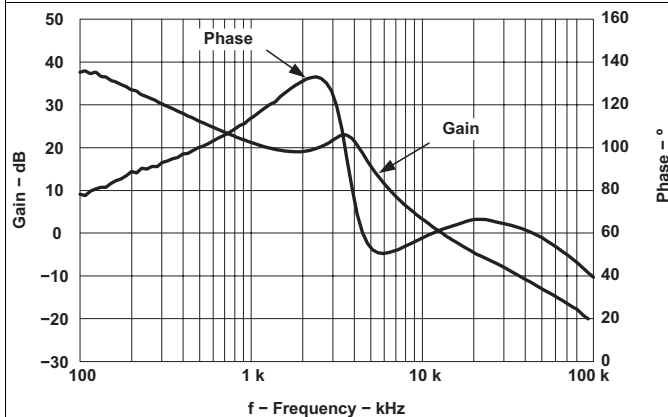
Figure 18. Overall Gain and Phase vs. Frequency
