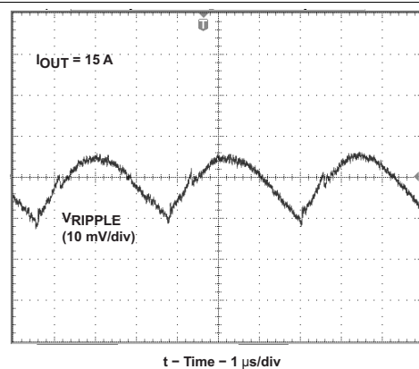
Figure 19. Output Voltage Ripple
