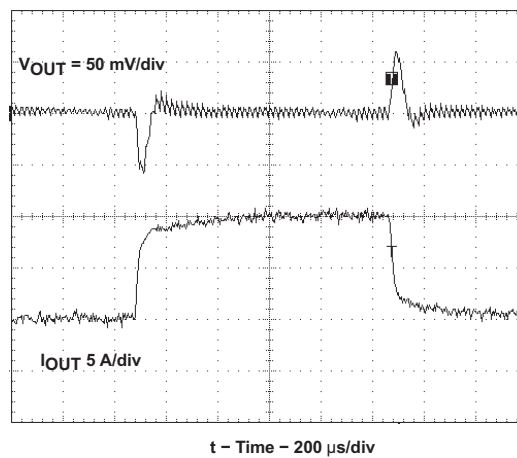
Figure 20. Transient Response
