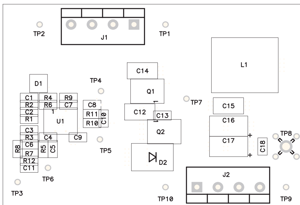
Figure 21. Top Side Component Assembly
