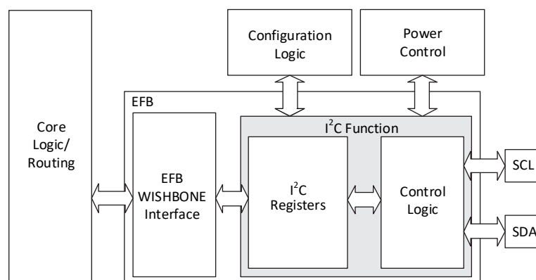
Figure 2.21. I²C Core Block Diagram
