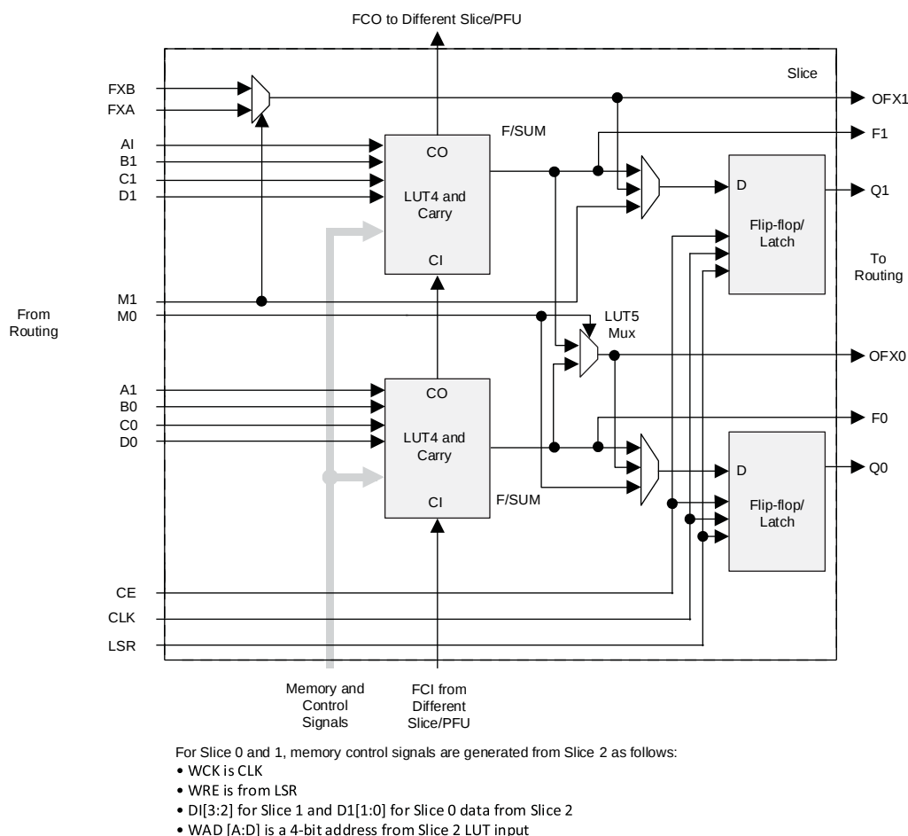
Figure 2.4. Slice Diagram
