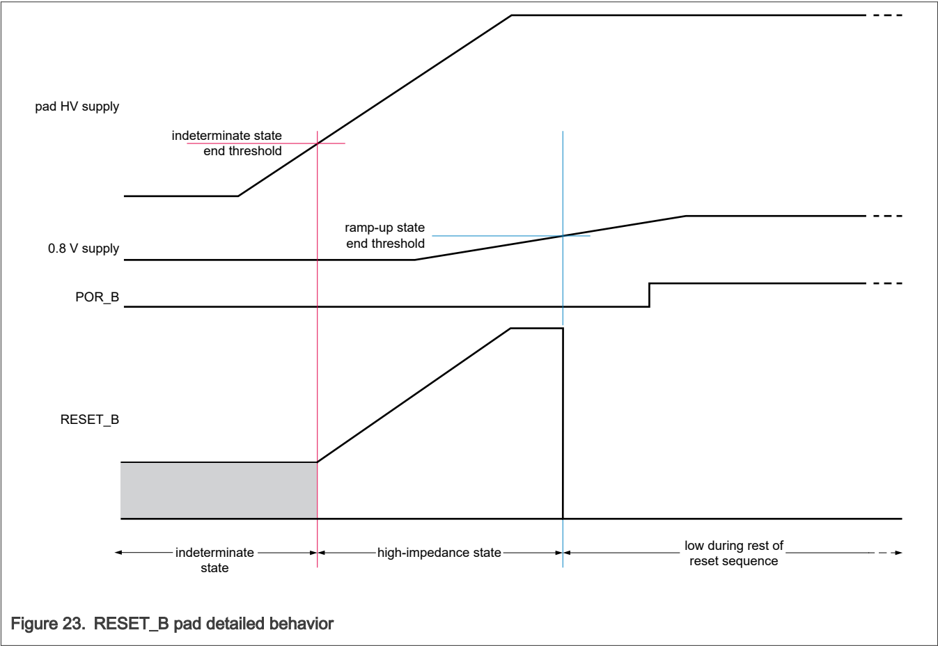
Figure 23. RESET_B pad detailed behavior The RESET_B pad behavior described in the diagram and the related VRSE_RESET_B parameter spec also apply to the case of core VDD droop after power-up.
