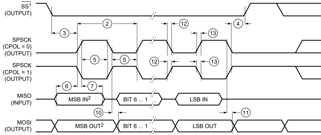
Figure 41. LPSPi Controller Mode Timing (CPHA=0)
