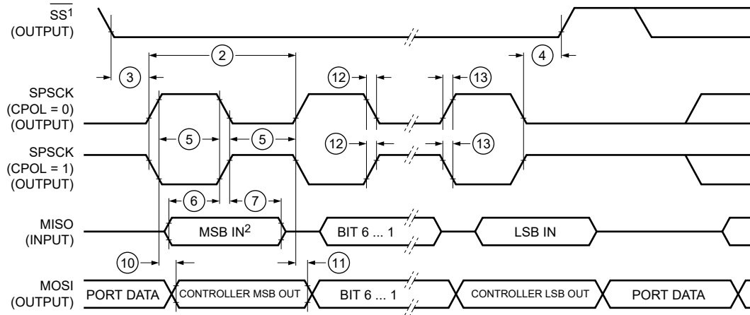
Figure 42. LPSPi Controller Mode Timing (CPHA=1)
