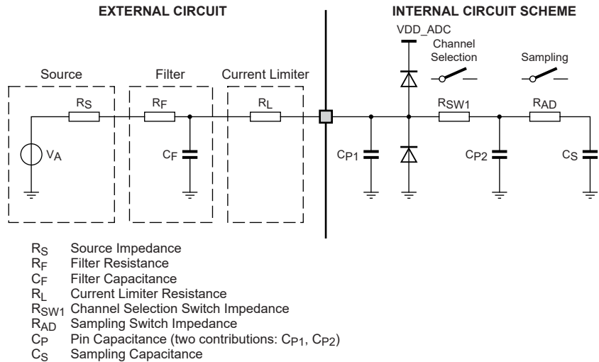
Figure 30. SAR ADC Input Circuit
