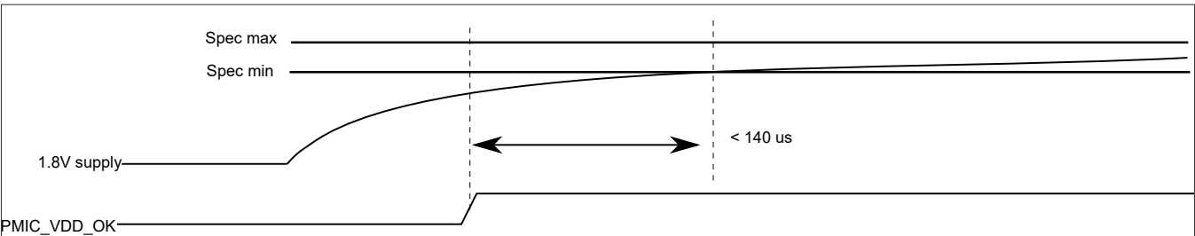
Figure 7. 1.8V supply timing with respect to PMIC_VDD_OK during Standby Mode Exit
