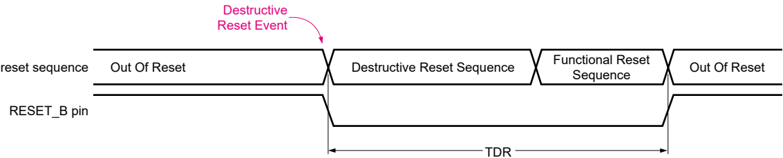
Figure 15. Destructive reset
