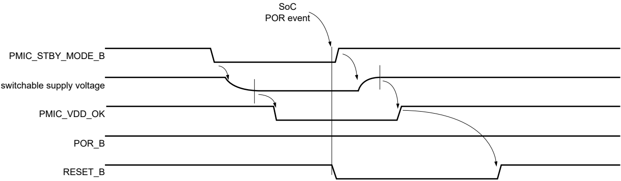
Figure 27. Standby Mode Aborted by SoC POR Event After PMIC_VDD_OK Deassertion
