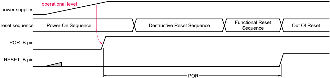
Figure 18. Initial power-up
