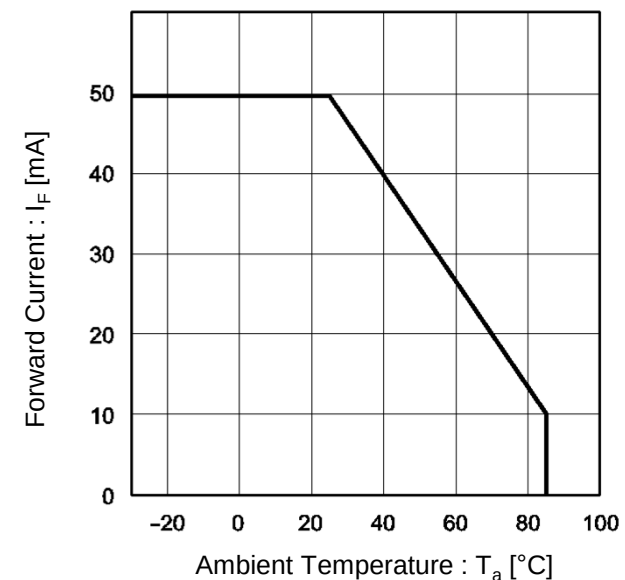
Fig.3 Forward Current Falloff
