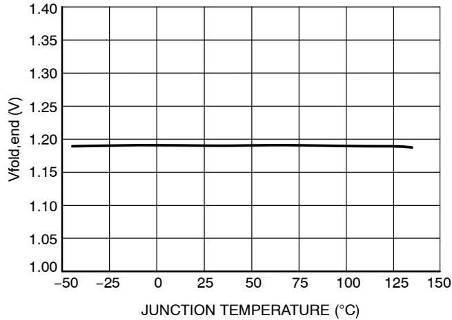
Figure 23. Vfold,end vs. Junction Temperature
