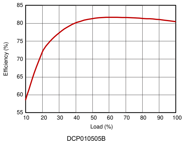
Figure 6-5. Efficiency versus Load
