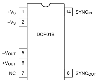
Figure 5-1. 7-Pin PDIP and SOP (Single Output) NVA and DUA Package (Top View)
