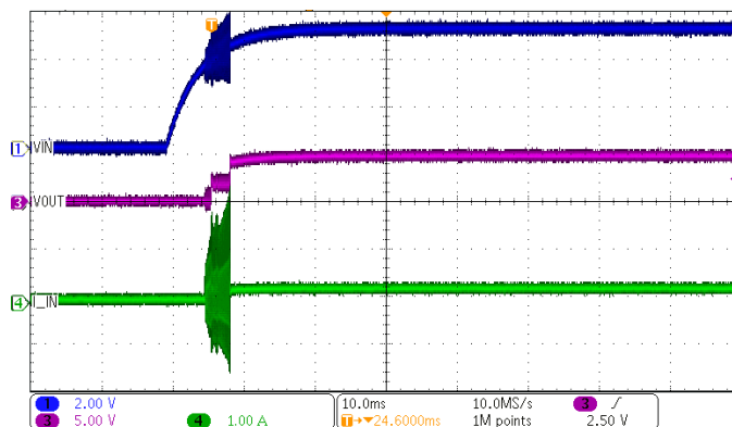
Figure 7-5. DCP010505BP Start-Up at 100% Load
