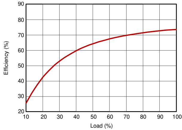
Figure 6-25. Efficiency versus Load
