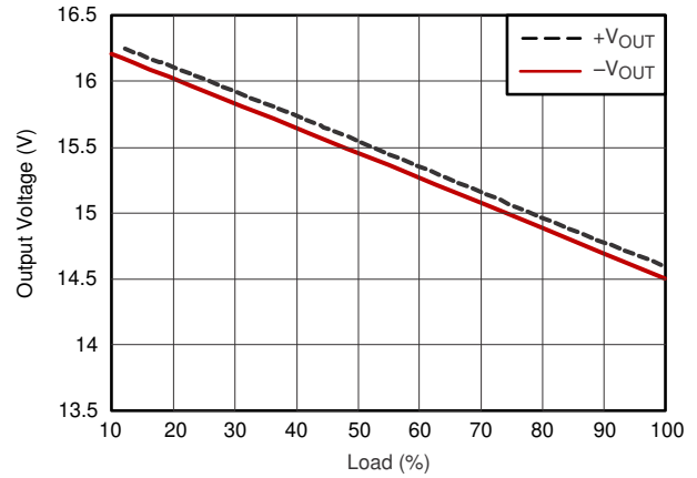
Figure 6-26. Load Regulation
