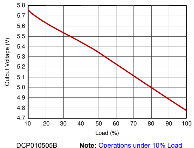
Figure 6-6. Load Regulation
