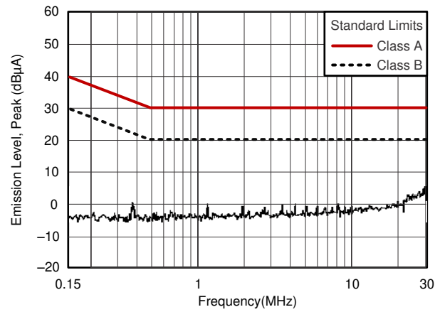
Figure 6-2. Conducted Emissions
