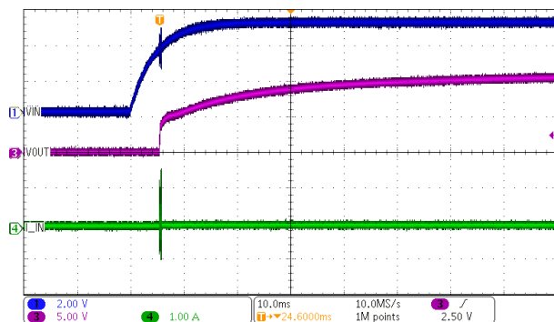
Figure 7-3. DCP010505BP Start-Up at No Load
