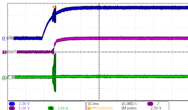
Figure 7-4. DCP010505BP Start-Up at 10% Load
