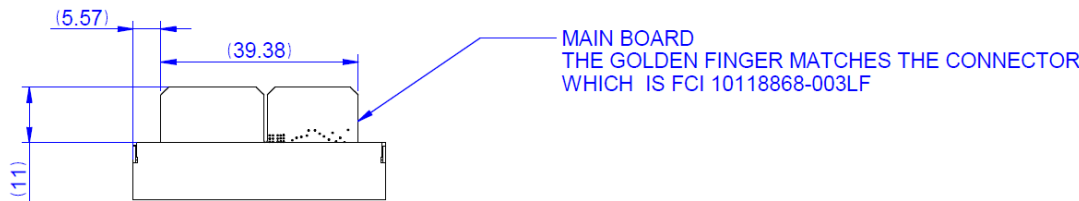
Figure 17. Mating Connector
