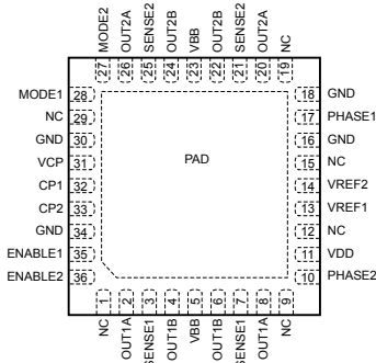
Pinout Diagram
