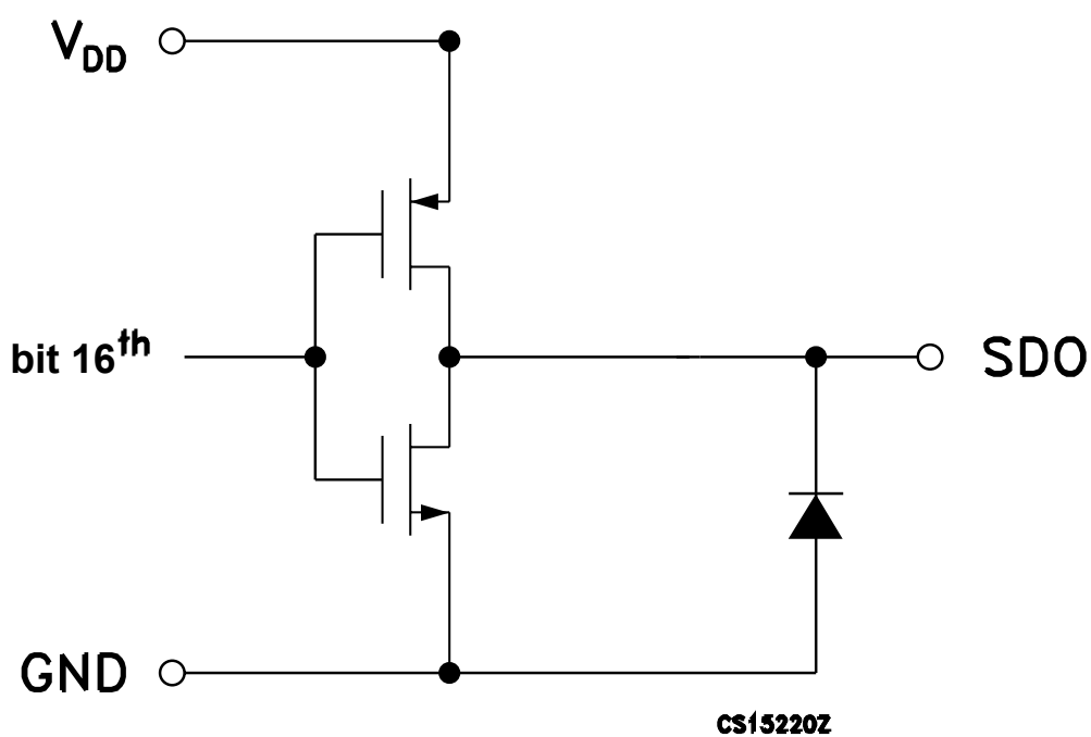
Figure 5. SDO terminal
