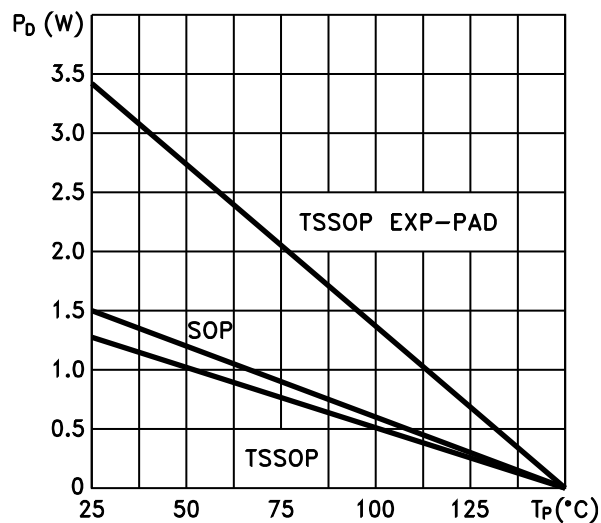
Figure 15. Power dissipation vs. package temperature
