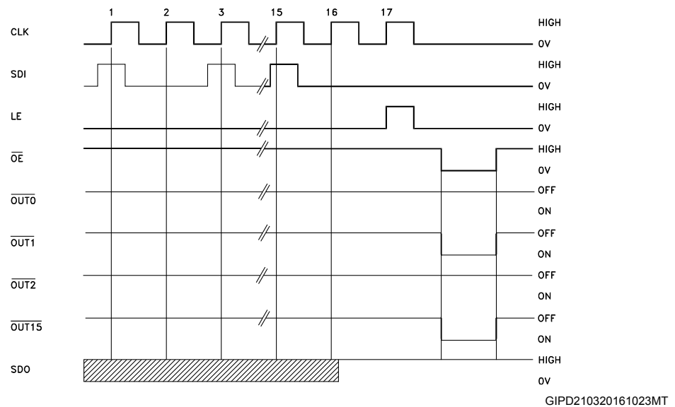
Figure 7. Timing diagram
