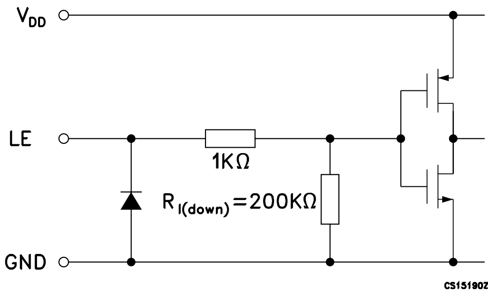
Figure 3. LE terminal
