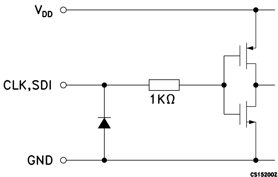
Figure 4. CLK, SDI terminal
