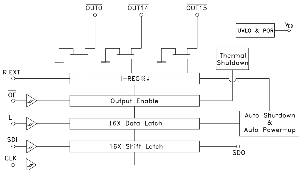
Figure 6. Block diagram
