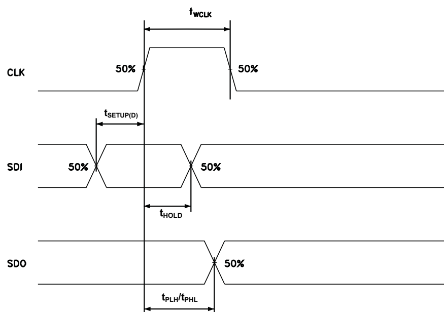
Figure 8. Clock, serial-in, serial-out
