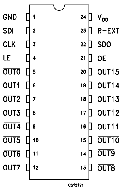
Figure 1. Pin connection
