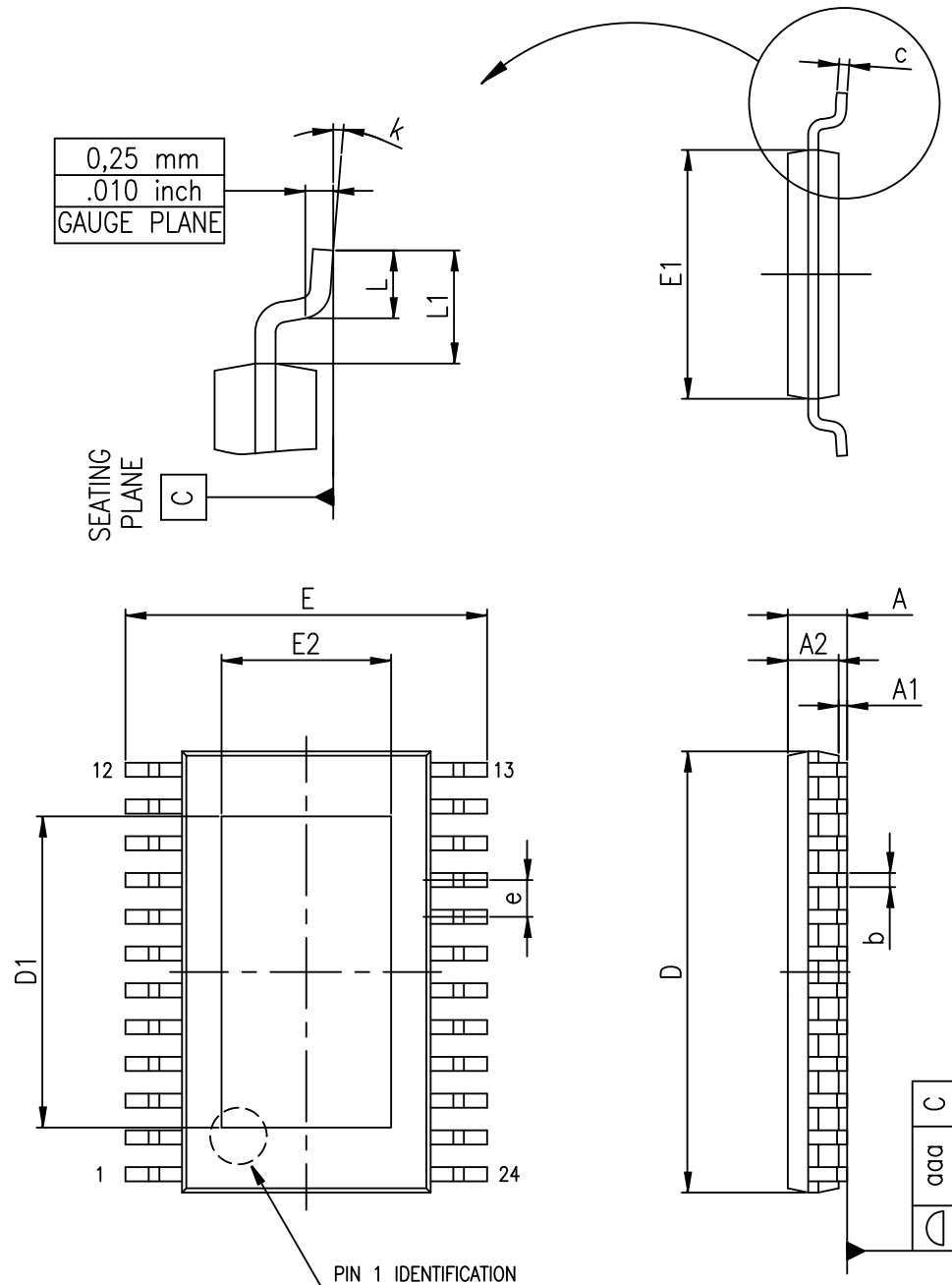
Figure 23. TSSOP24 exposed pad package outline
