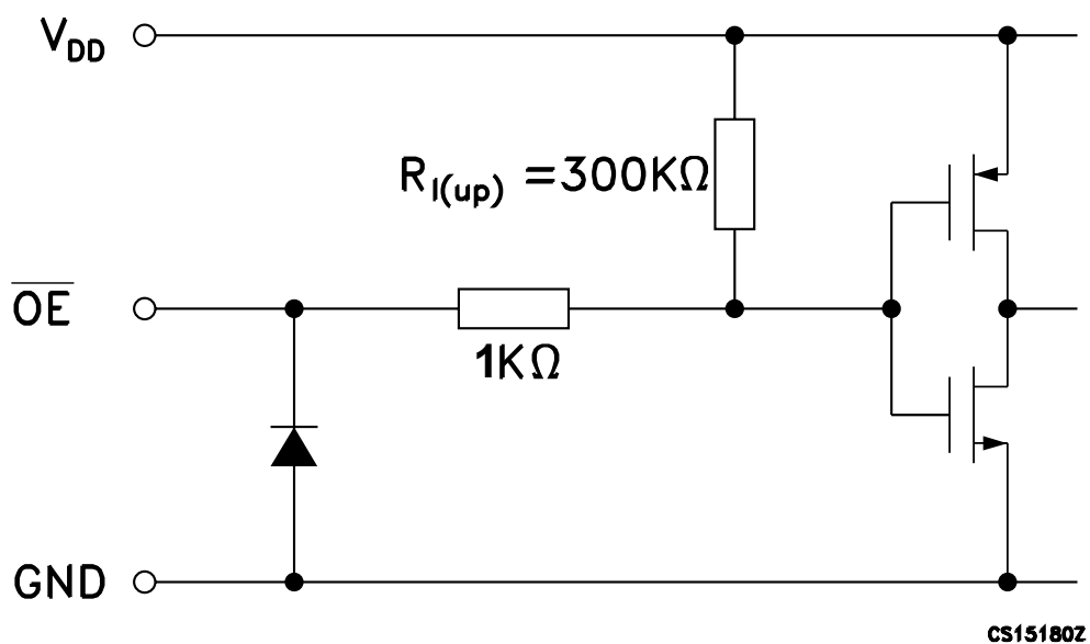
Figure 2. \overline{OE} terminal
