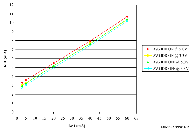
Figure 14. Idd ON/OFF
