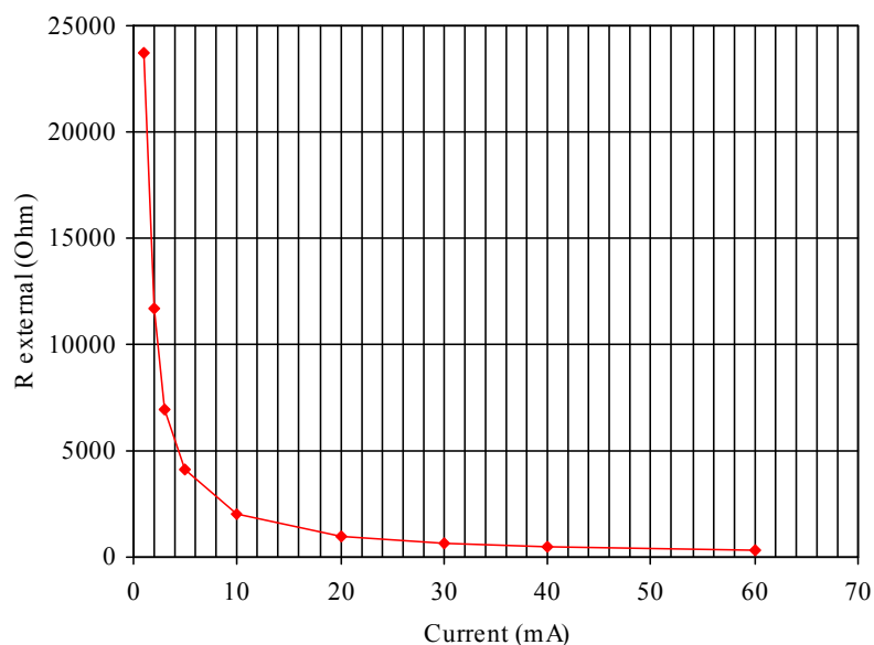
Figure 11. Output current vs. R-EXT resistor
