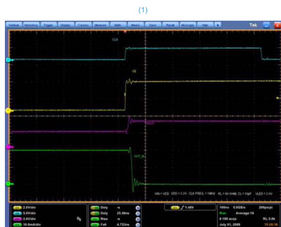
Figure 16. Turn ON output current characteristics
