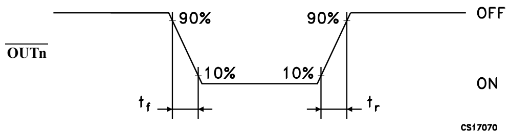
Figure 10. Outputs
