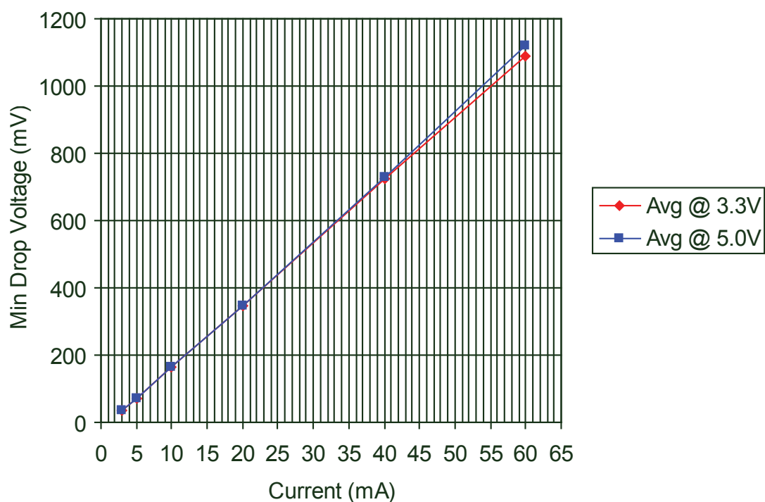
Figure 12. I_{SET} vs drop out voltage ( V_{drop} )
