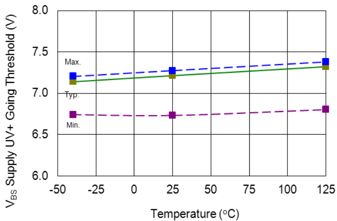
Figure 34. VBS UV+ Going Threshold vs. Temperature
