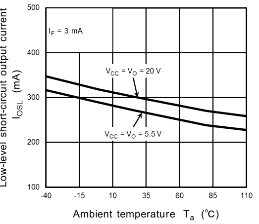
Fig. 12.2.9 I_{osL} - T_a
