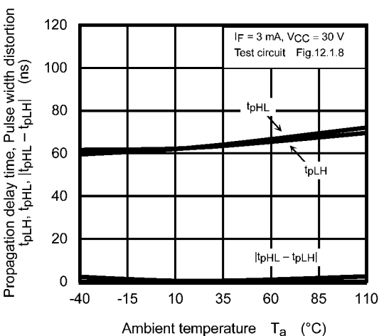
Fig. 12.2.14 t_{pLH} , t_{pHL} , |t_{pHL} - t_{pLH}| - T_a (Test Circuit Fig. 12.1.8)
