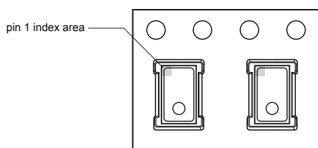
Figure 15. Device orientation in chip carrier
