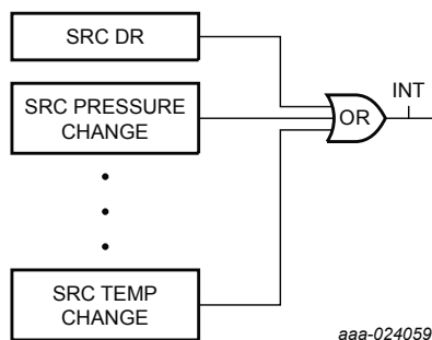
Figure 10. INT1/INT2 pin control logic
