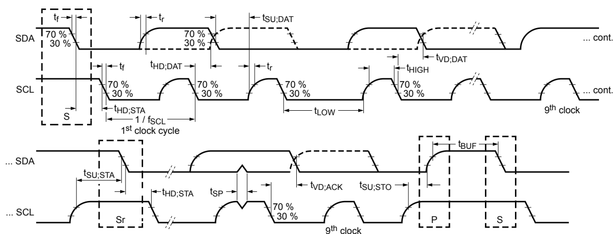
Figure 4. I 2 C client timing diagram
