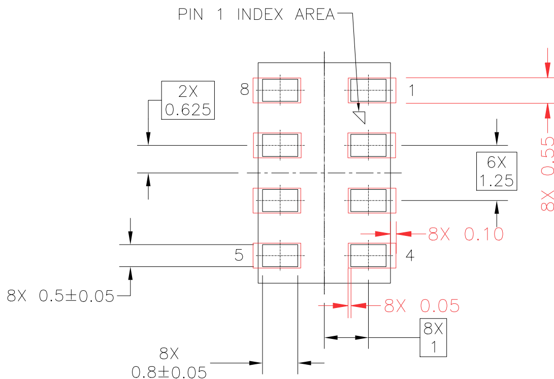
Figure 13. Recommended PCB landing pattern
