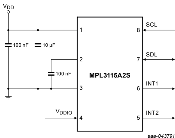
Figure 3. Typical application diagram
