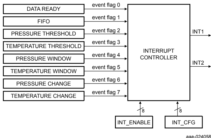
Figure 9. Interrupt controller block diagram
