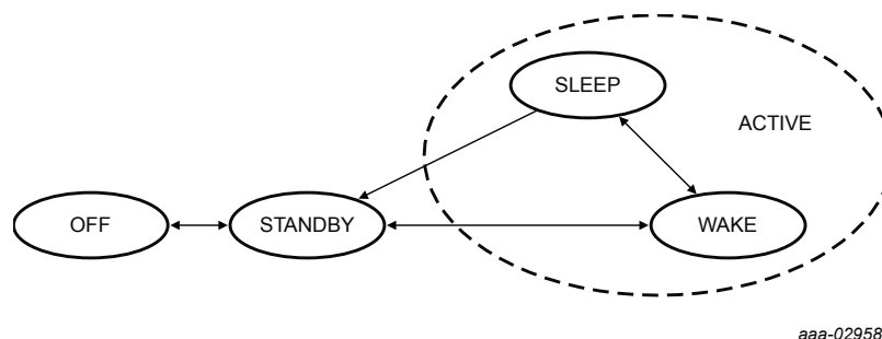
Figure 6. Mode transition diagram
