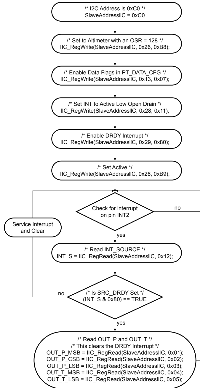
Figure 8. Interrupt - no FIFO
