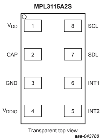
Figure 2. 8-pin LGA pinout
