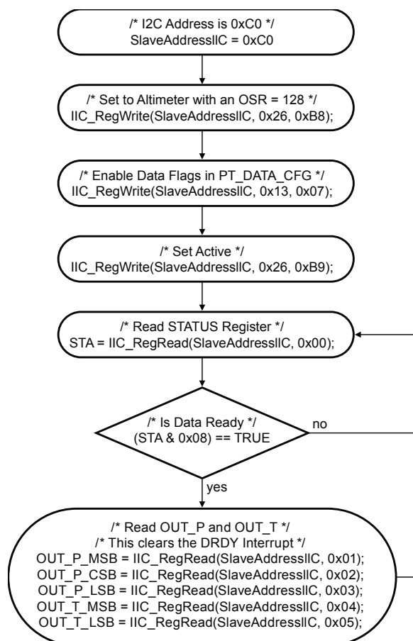
Figure 7. Polling - no FIFO
