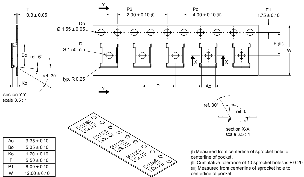
Figure 14. LGA 3 mm × 5 mm embossed carrier tape dimensions
