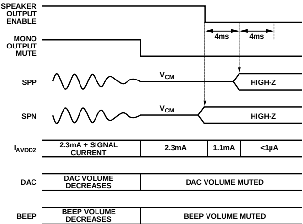
Figure 36. Speaker Driver Power-Down Sequence
