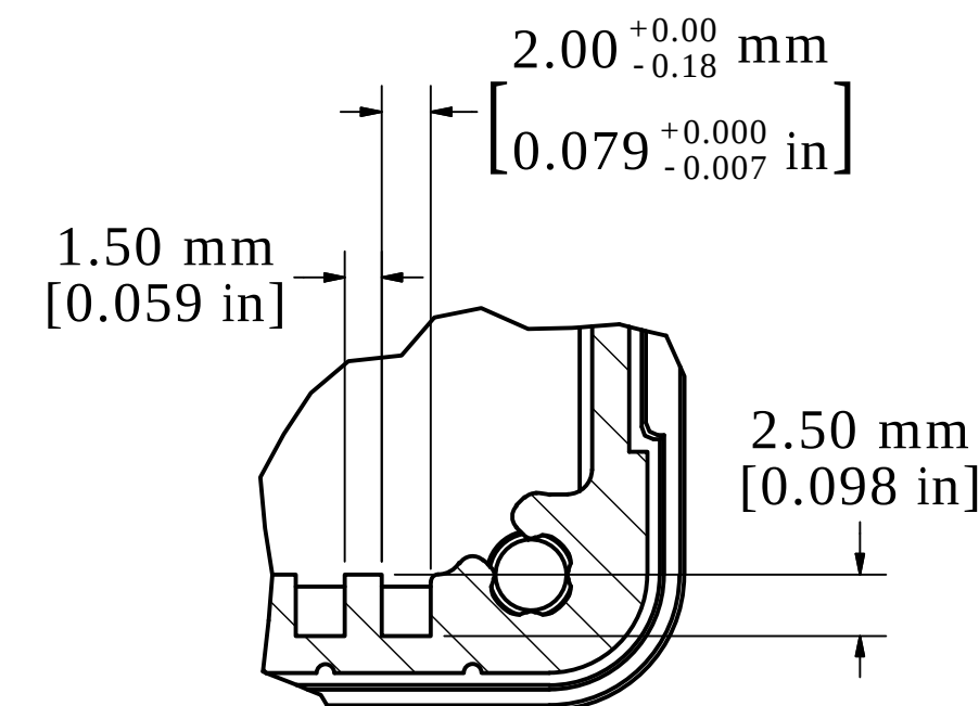
DETAIL W
