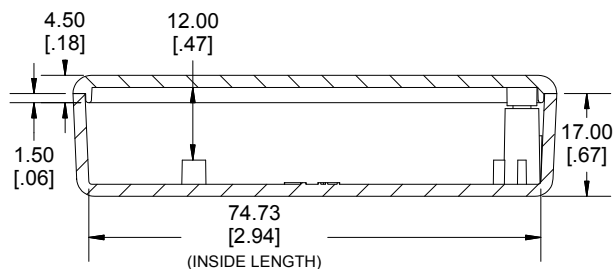
SIDE VIEW SECTION A-A
