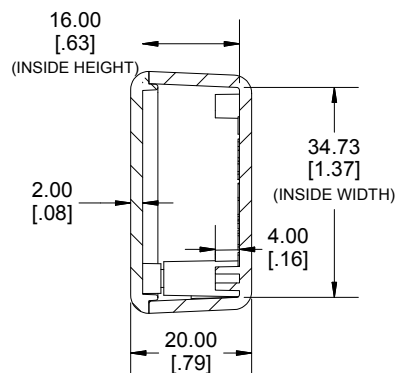
END VIEW SECTION B-B
