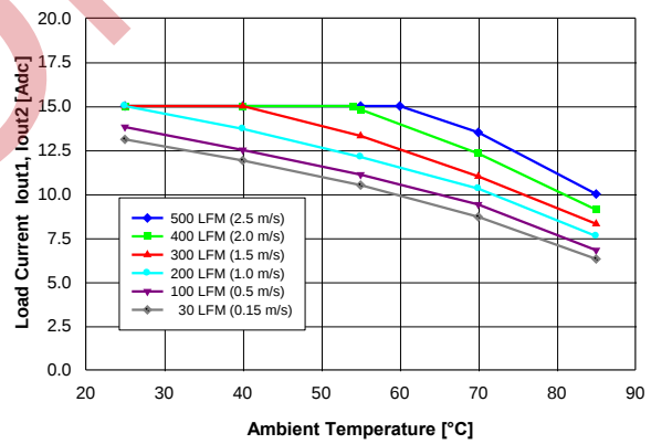
Figure 10. Available balanced load current ( I_{out1} = I_{out2} ) vs. ambient air temperature and airflow rates for converter mounted horizontally with V_{in} = 48\text{ V} , air flowing from pin 3 to pin 4 and maximum FET temperature \leq 120\text{ }^{\circ}\text{C} .
