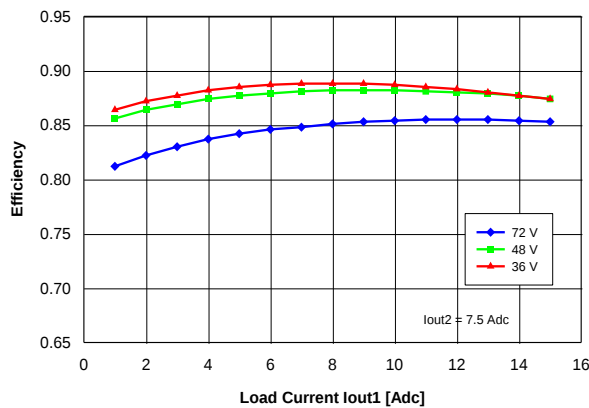
Figure 11. Efficiency vs. load current I_{out1} and input voltage for converter mounted vertically with air flowing from pin 3 to pin 1 at a rate of 300 LFM (1.5 m/s), for I_{out2} = 7.5 A and T_a = 25 °C.
