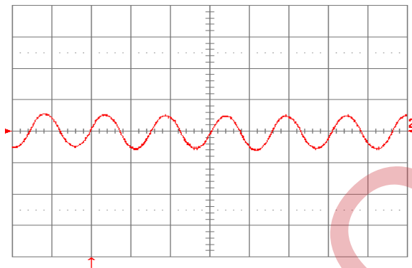
Figure 31. Input reflected ripple current, i_c (100 mA/div), measured at input terminals at full rated load current on both outputs and V_{in} = 48\text{ V} . Refer to Fig. 30 for test setup. Time scale: 1 \mu\text{s}/\text{div} .
