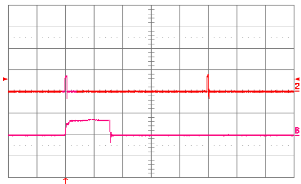
Figure 28. Load current Iout2 into a 10 m \Omega short circuit on Vout2 during restart, with Vout1 open (no load), at V_{in} = 48 V. Ch2 = Iout2 (20 A/div, 20 ms/div). ChB = Iout2 (20 A/div, 1 ms/div) is an expansion of the on-time portion of Iout2.
