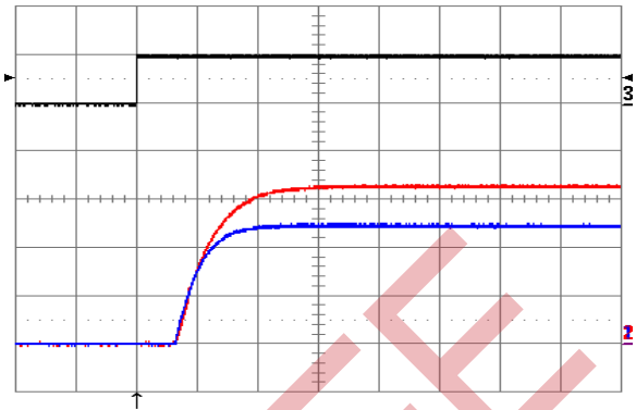
Figure 18. Turn-on transient waveforms at full rated load current (resistive) and V_{in} = 48\text{ V} , triggered via ON/OFF pin. Top trace: ON/OFF signal (5 V/div.). Bottom traces: Vout1 (blue, 1 V/div.), Vout2 (red, 1 V/div.). Time scale: 1 ms/div..
