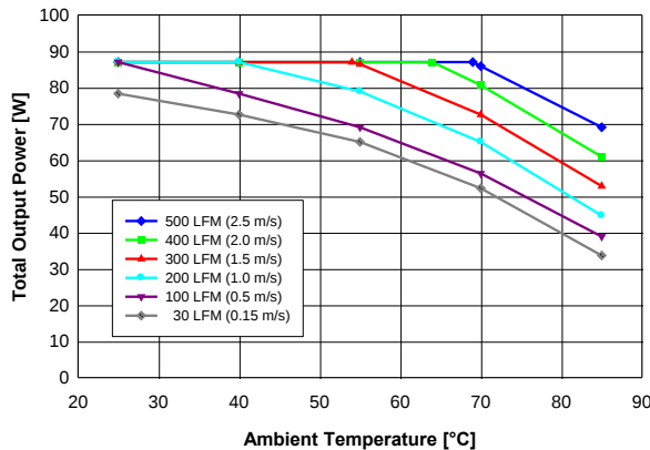
Figure 7. Available output power for balanced load current ( I_{out1} = I_{out2} ) vs. ambient air temperature and airflow rates for converter mounted vertically with V_{in} = 48\text{ V} , air flowing from pin 3 to pin 1 and maximum FET temperature \leq 120\text{ }^{\circ}\text{C} .
