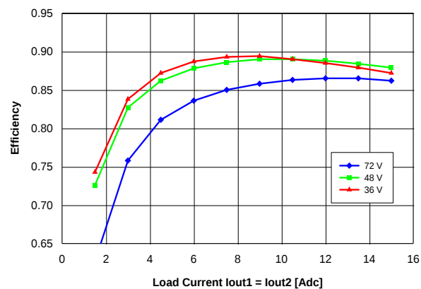
Figure 16. Efficiency vs. balanced load current ( I_{out1} = I_{out2} ) and input voltage for converter mounted horizontally with air flowing from pin 3 to pin 4 at a rate of 300 LFM (1.5 m/s) and T_a = 25 °C.
