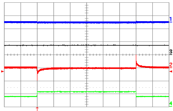
Figure 22. Output voltage response to Iout2 load current step-change of 3.75 A (50%-75%-50%) at Iout1 = 7.5 A and V_{in} = 48\text{ V} . Ch1 = Vout1 (100 mV/div), Ch2 = Vout2 (100 mV/div), Ch3 = Iout1 (10 A/div.), Ch4 = Iout2 (10 A/div.). Current slew rate: 5\text{ }\mu\text{A/s} , C_o = 300\text{ }\mu\text{F} tantalum + 1\text{ }\mu\text{F} ceramic. Time scale: 0.5 ms/div.
