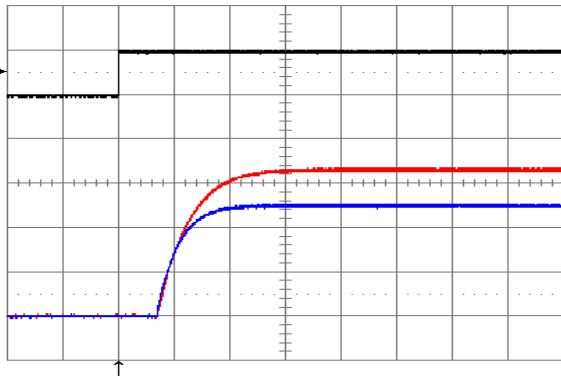
Figure 17. Turn-on transient waveforms at no load current and V_{in} = 48\text{ V} , triggered via ON/OFF pin. Top trace: ON/OFF signal (5 V/div.). Bottom traces: Vout1 (blue, 1 V/div.), Vout2 (red, 1 V/div.). Time scale: 1 ms/div.
