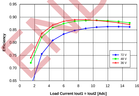
Figure 15. Efficiency vs. balanced load current ( I_{out1} = I_{out2} ) and input voltage for converter mounted vertically with air flowing from pin 3 to pin 1 at a rate of 300 LFM (1.5 m/s) and T_a = 25 °C.
