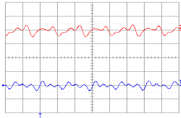
Figure 29. Output voltage ripple at full rated load current into a resistive load on both outputs with C_o = 1\mu\text{F} (ceramic) and V_{in} = 48\text{ V} . Ch2 = Vout2, Ch1 = Vout1 (both 20 mV/div). Time scale: 1 \mu\text{s}/\text{div} .
