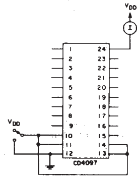
Fig. 10—Quiescent device current.
