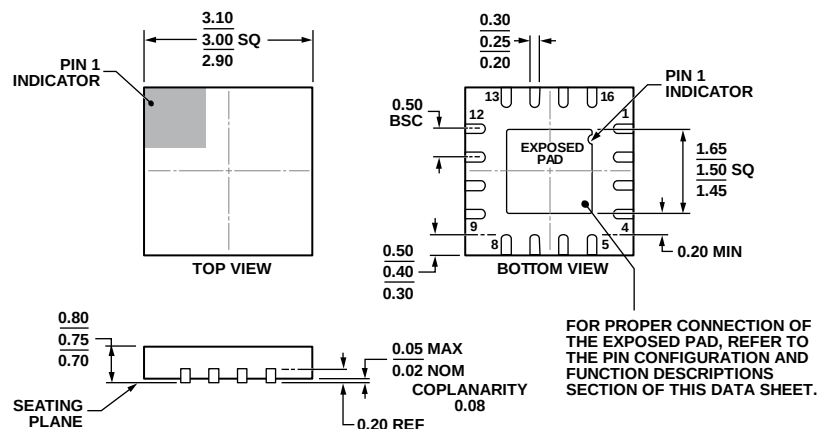
Figure 36. 16-Lead Lead Frame Chip Scale Package [LFCSP] 3 mm × 3 mm Body and 0.75 mm Package Height (CP-16-27)
