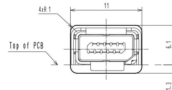
4 Reference Dimensions of Panel Cutout (Free)
