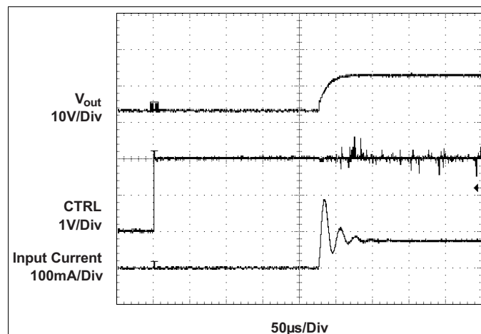
Figure 16. Soft-Start
