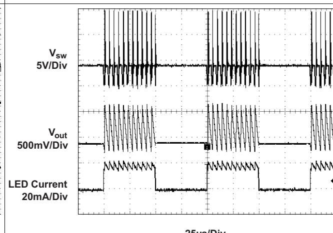
Figure 19. PWM Dimming
