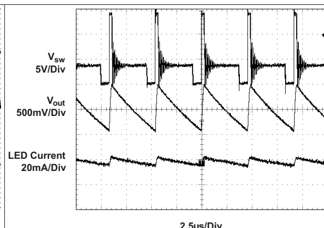
Figure 17. PFM Operation
