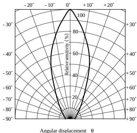
Fig. 9 Sensitivity Diagram ( T_a = 25^\circ C )
