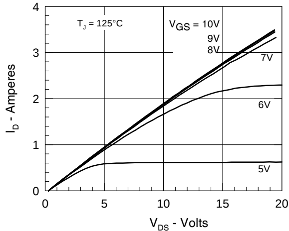
Figure 3. Output characteristics at 125°C
