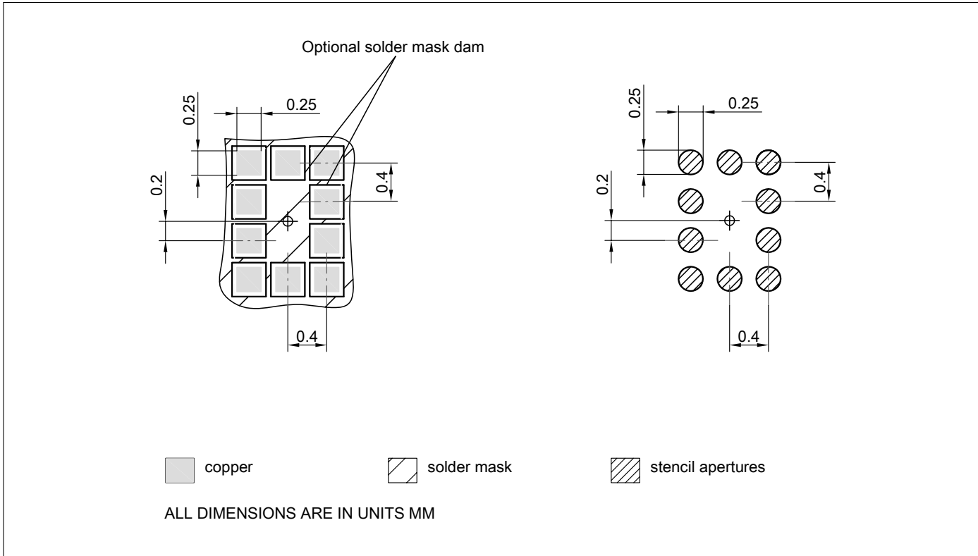
Figure 7: Footprint Recommendation
