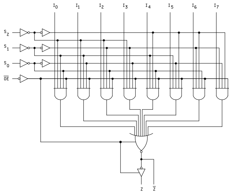
FIGURE 3. Logic diagram.
