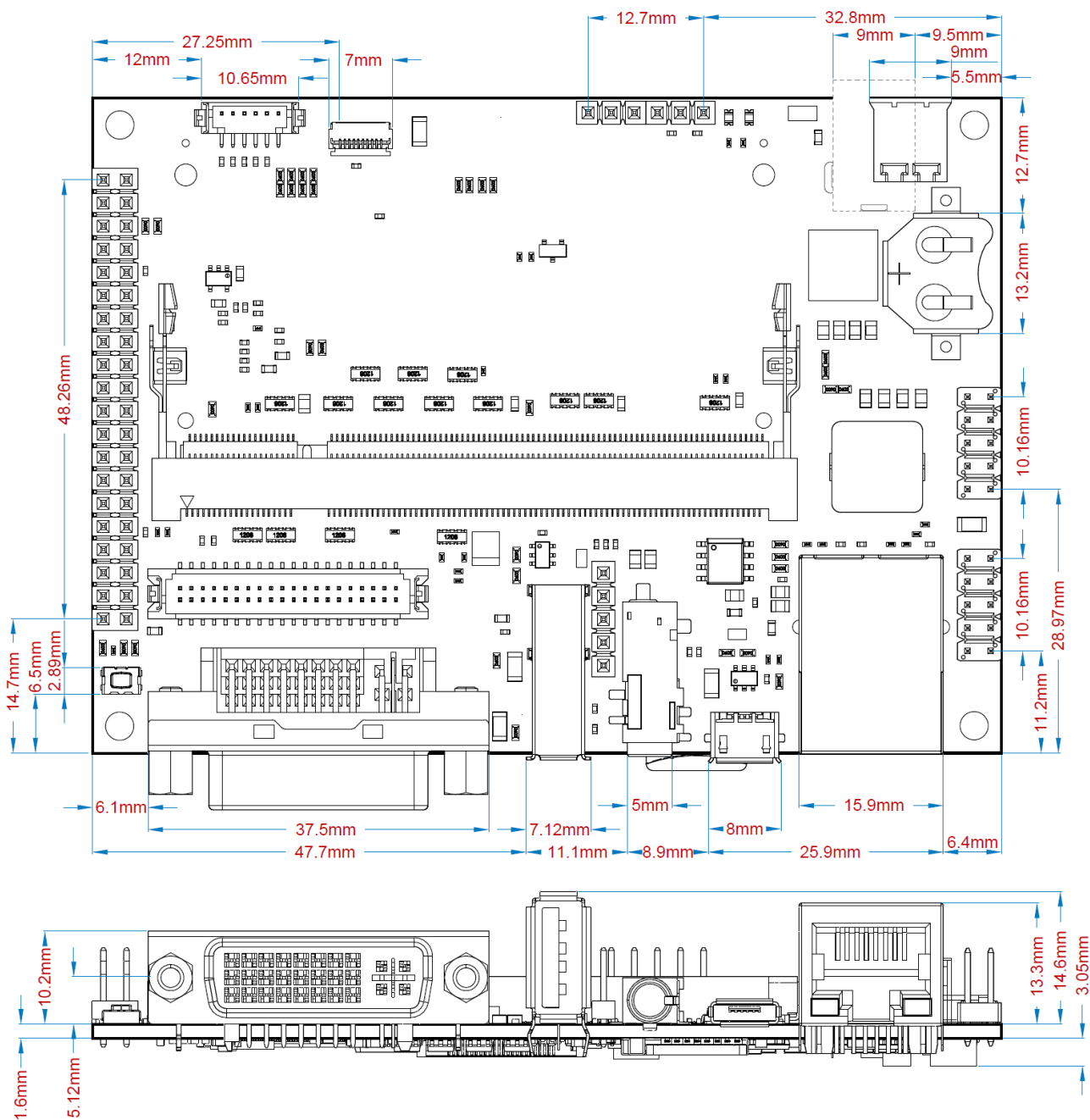
Fig.7 Iris Dimensions – Top Side, all dimensions are in millimetres (mm)
