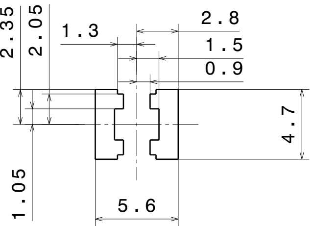
Recommended PAD design
