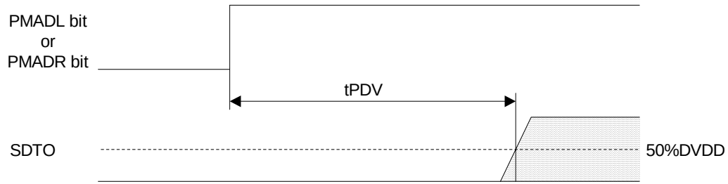
Figure 11. Power Down &amp; Reset Timing 1
