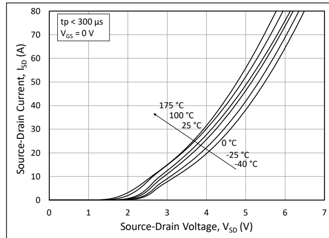
Figure 6. 3 rd Quadrant Characteristic vs. Junction Temperatures at V_{GS} = 0\text{ V}
