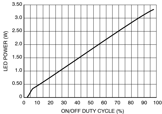
Figure 26. Dimming Characteristic
