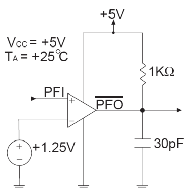
Fig. 7: Power-Fail Comparator Assertion Response Time Circuit
