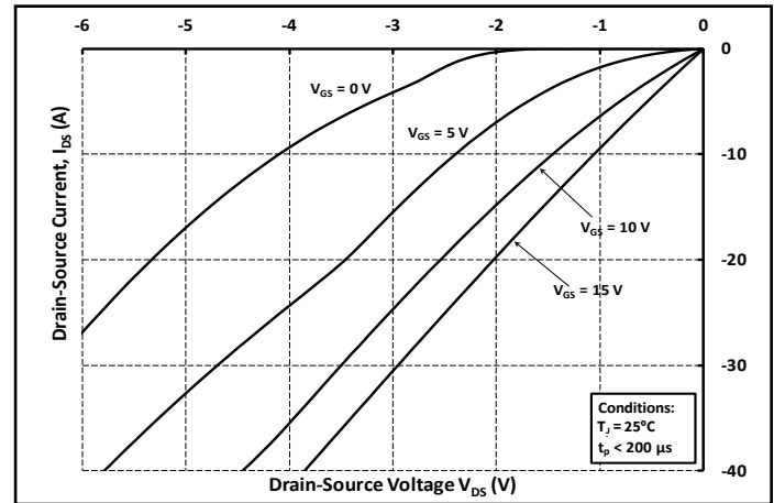
Figure 14. 3rd Quadrant Characteristic at 25^{\circ}\text{C}
