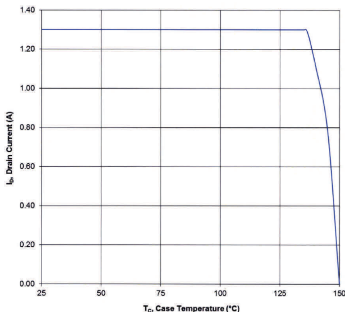
Fig 1. Maximum Drain Current Vs Case Temperature
