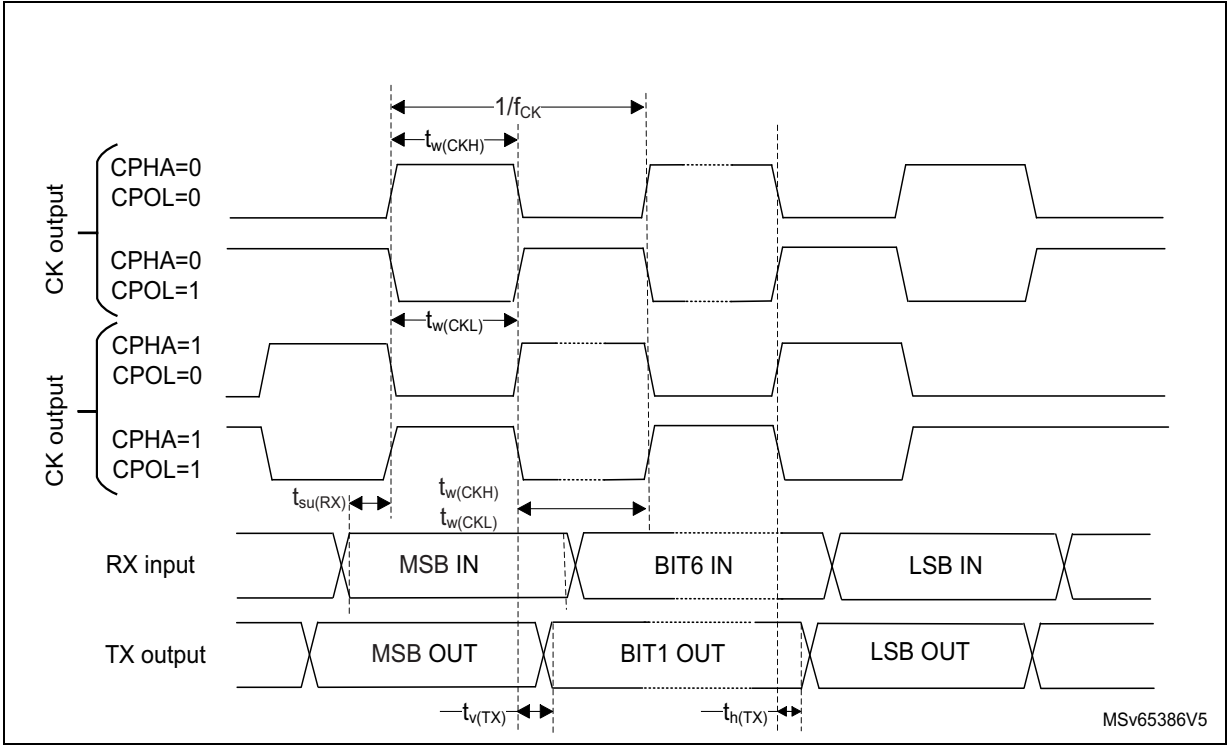
Figure 81. USART timing diagram in master mode
