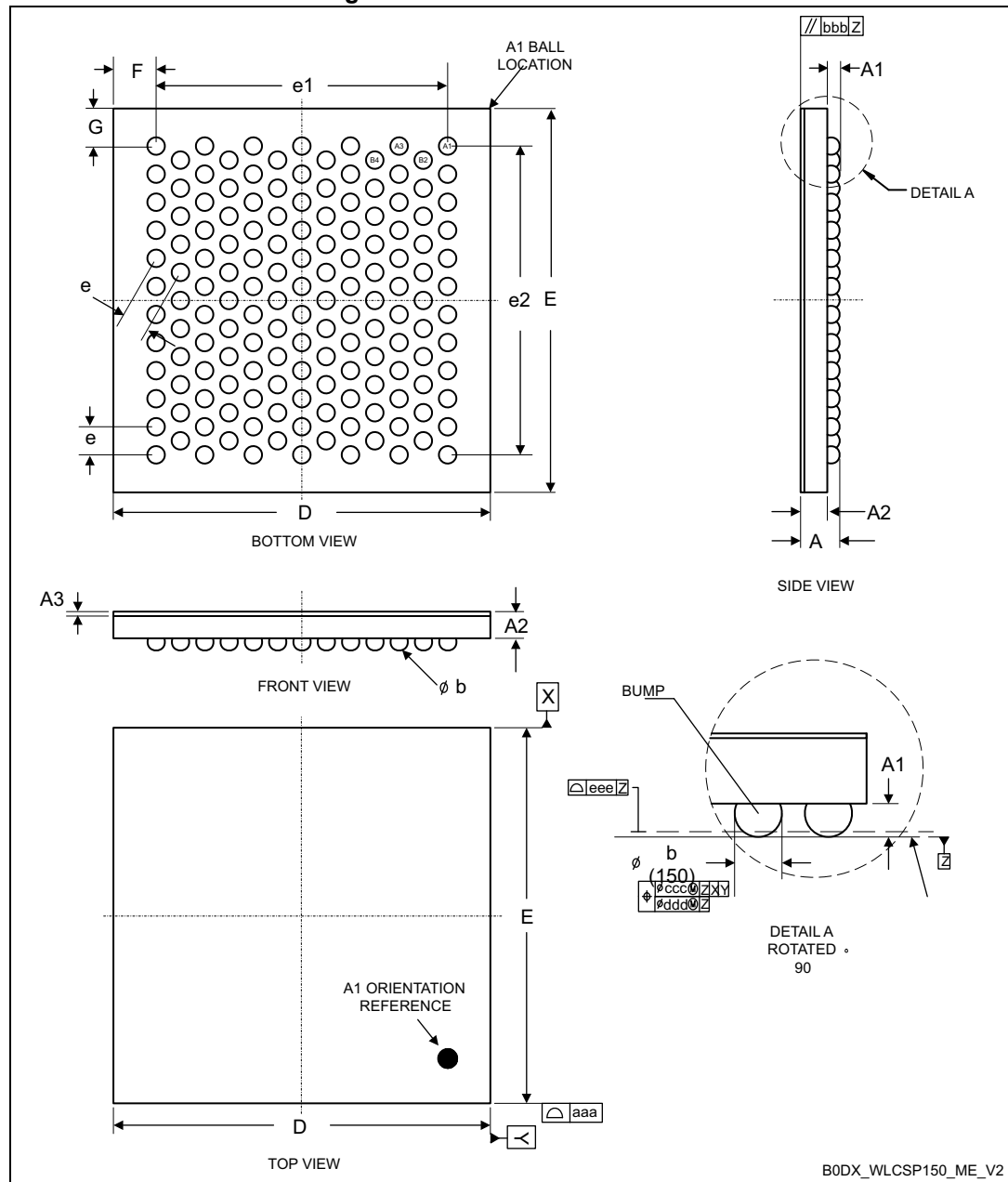
Figure 102. WLCSP150 - Outline
