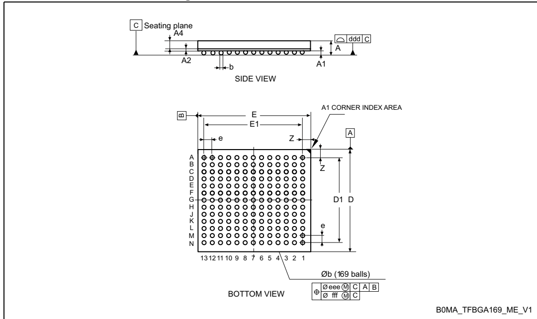
Figure 105. TFBGA169 - Outline
