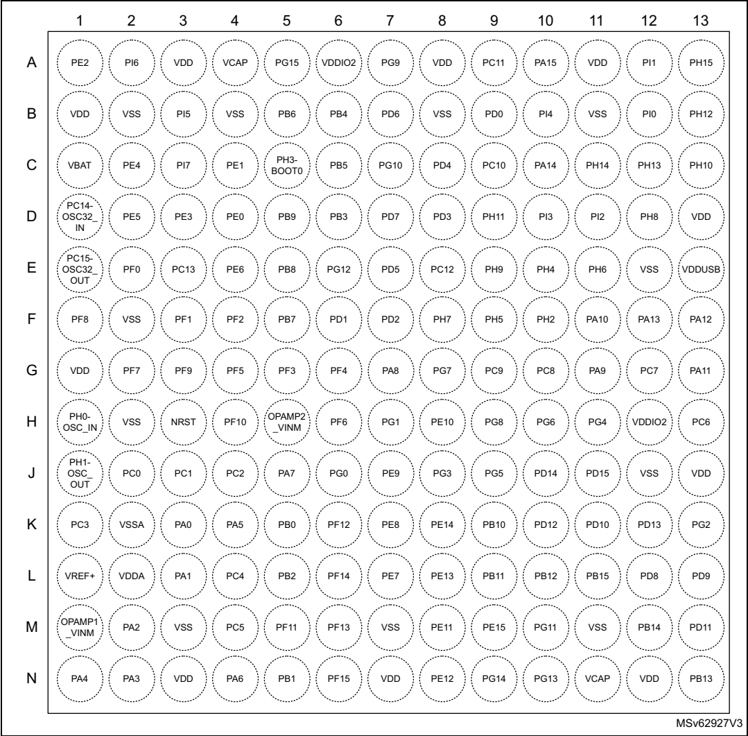
Figure 18. TFBGA169 ballout
