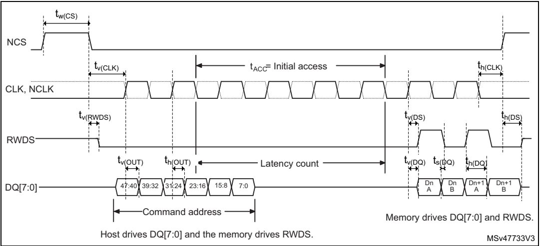
Figure 70. OCTOSPI HyperBus read
