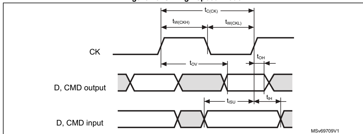
Figure 79. SD default mode
