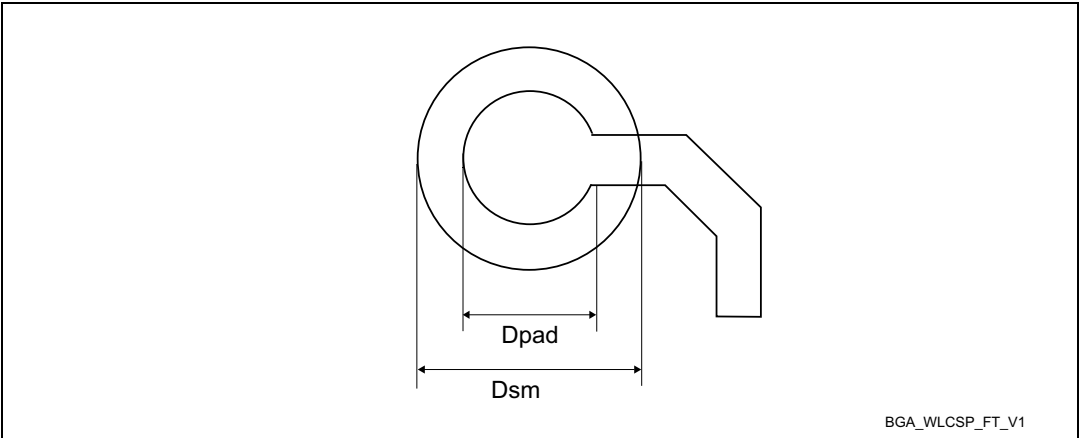
Figure 103. WLCSP150 - Recommended footprint
