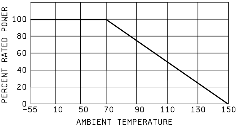
FIGURE 2. Derating curve .
