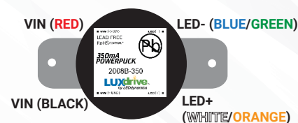
Figure 2. Wire Configuration
