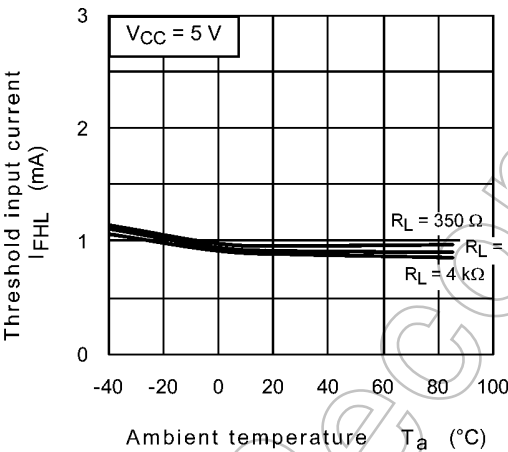
Fig. 13.2.3 I_{FHL} - T_a
