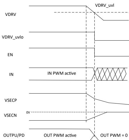
Figure 5: Shutdown Mechanism
