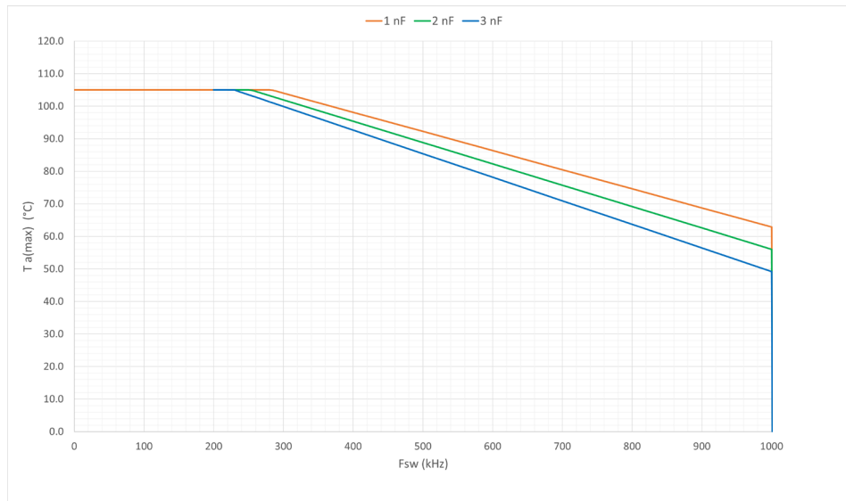
Figure 9: AHV85111 thermal derating curve as a function of load capacitance C_{OUT} and PWM frequency f_{SW}
