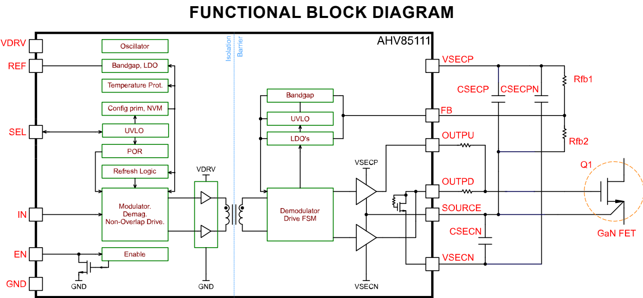
Figure 2: AHV85111 Block Diagram
