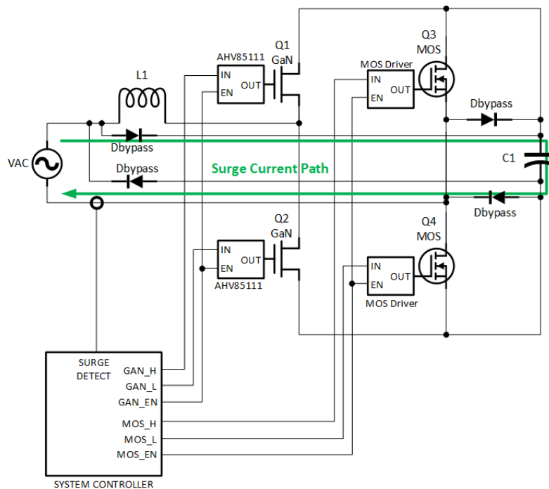
Figure 12: Block diagram of system level surge-detection inhibit signal; used to disable isolated gate drivers using the EN pins
