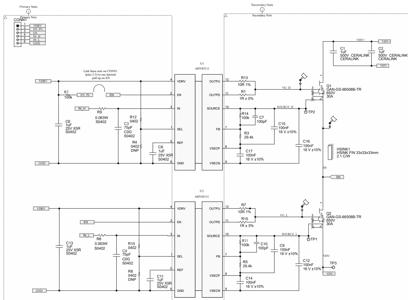
Figure 10: APEK85111KNH-02-T-MH schematic for driving a GaN transistor with a bipolar drive arrangement.
