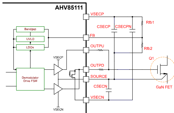
Figure 7: Rfb1 and Rfb2 used to set the desired VSECP-to-SOURCE positive bias rail regulation level
