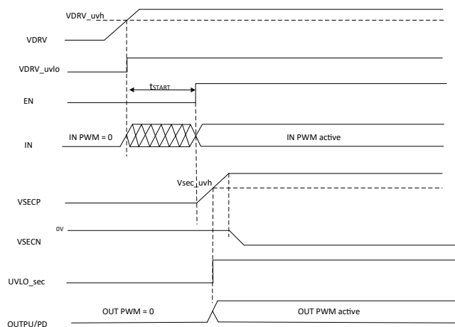
Figure 4: AHV85111 Startup Mechanism
