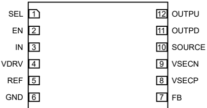
Package NH Pinout (Top View)
