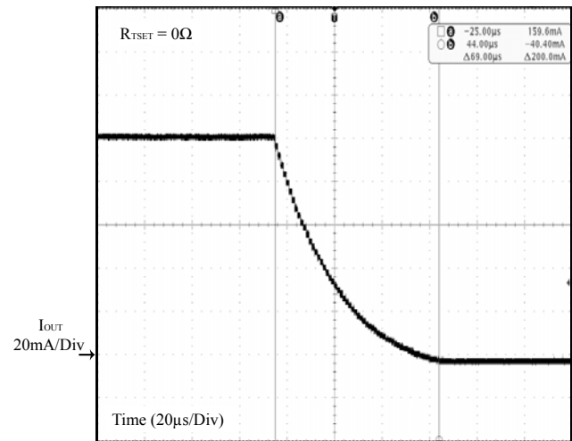
Figure 11 Instant Off
