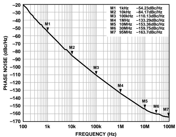
Figure 9. Open-Loop VCO Phase Noise, 8.0 GHz, VCC_VCO = 5 V
