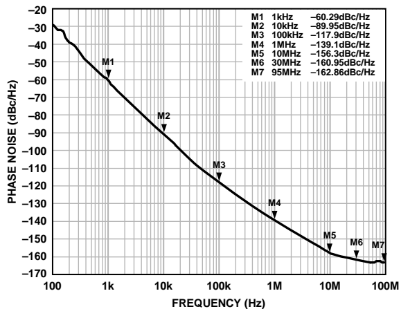
Figure 7. Open-Loop VCO Phase Noise, 4.0 GHz, VCC_VCO = 5 V
