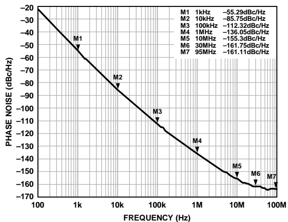
Figure 8. Open-Loop VCO Phase Noise, 5.7 GHz, VCC_VCO = 5 V
