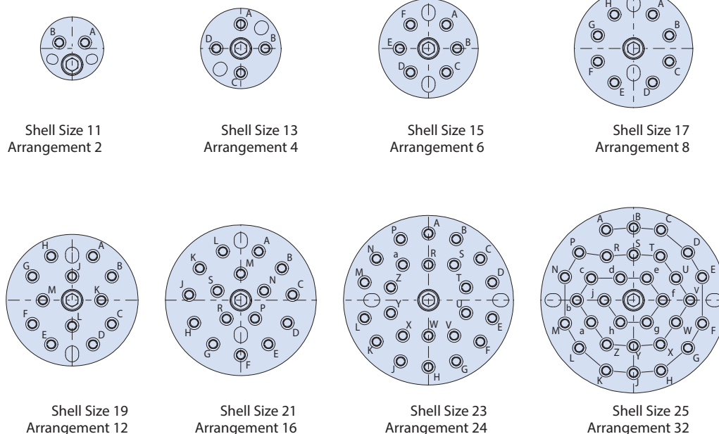
Figure 1: Insert Arrangements ASR Face Shown
