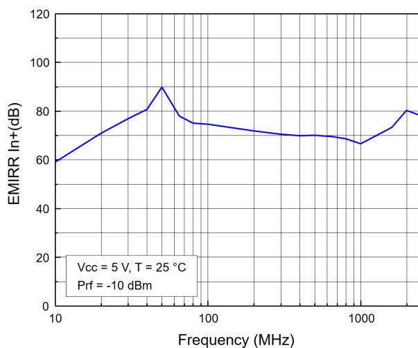
Figure 45. EMIRR on pin+
