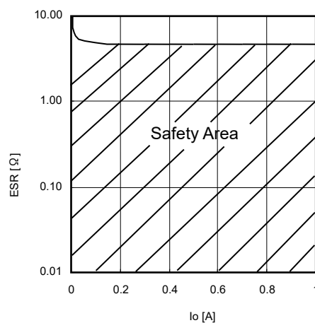
ESR – I_O characteristics
