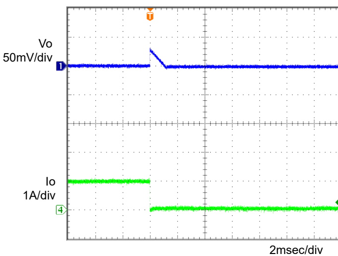
Fig.6 Transient Response (1.0→0A) Co=1\mu F, Ta=-40^{\circ}C
