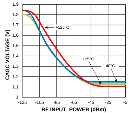
CAGC Voltage vs. Input Power
