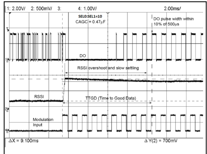
Figure 4. RSSI Overshoot and Slow TTGD (9.1ms)
