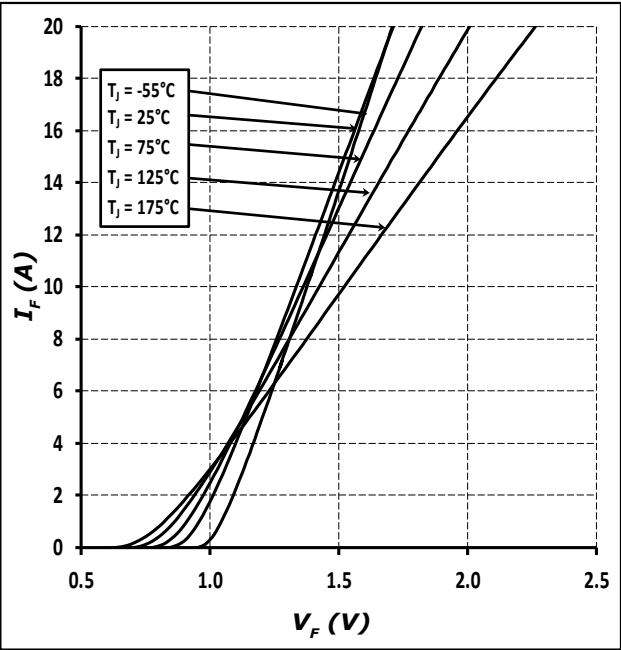
Figure 1. Forward Characteristics
