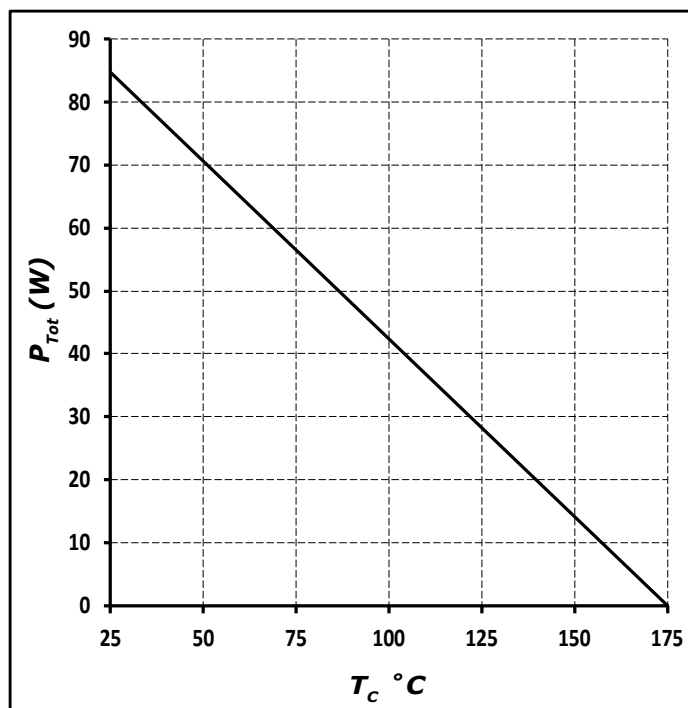
Figure 4. Power Derating
