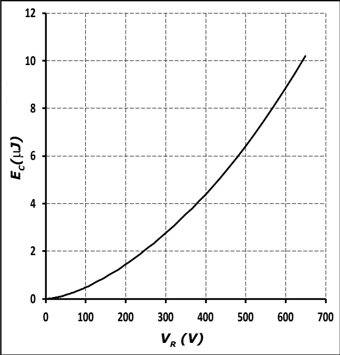
Figure 7. Capacitance Stored Energy
