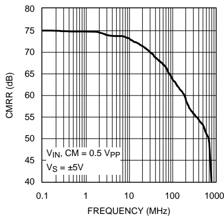
Figure 21. CMRR
