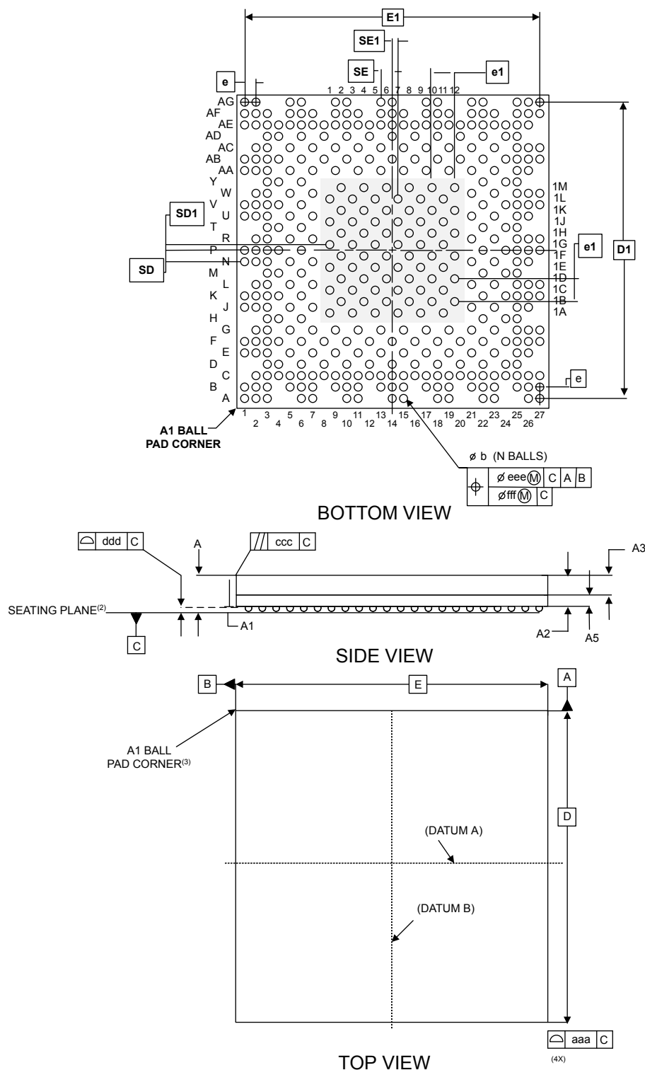
Figure 65. VFBGA424 - Outline
