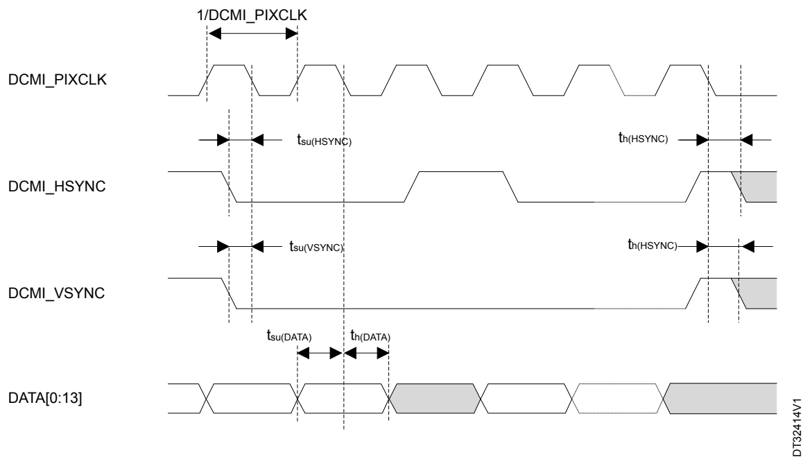
Figure 41. DCMI timing diagram
