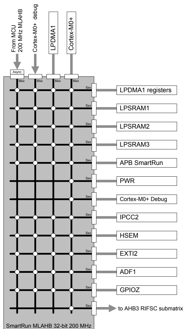
Figure 5. SmartRun multi-Layer AHB matrix
