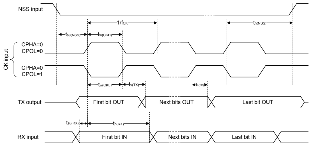
Figure 61. USART timing diagram in SPI slave mode
