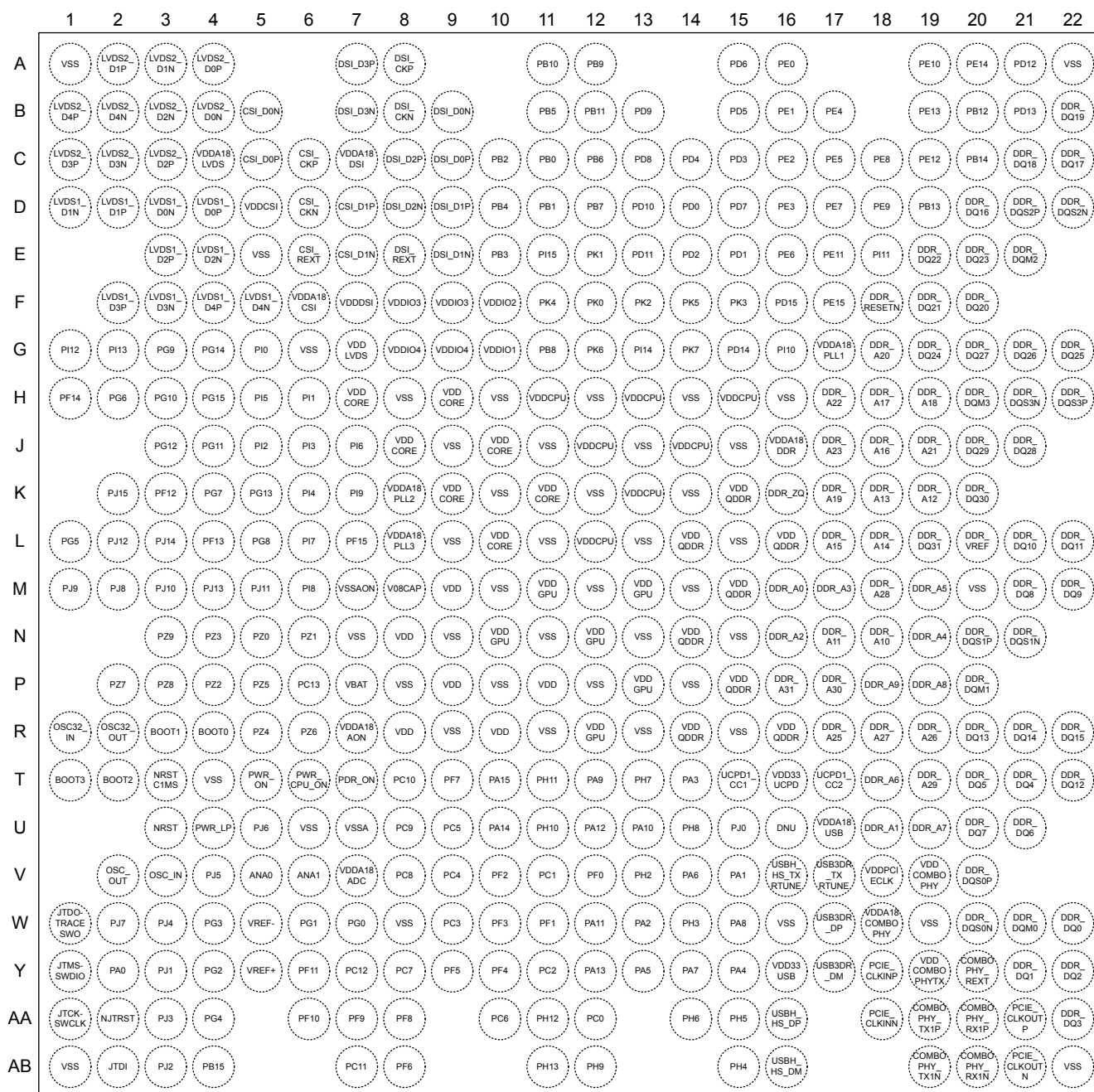
Figure 8. STM32MP25xC/F TFBGA436 pinout
