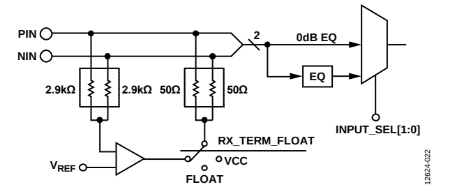
Figure 22. Input Stage Block Diagram
