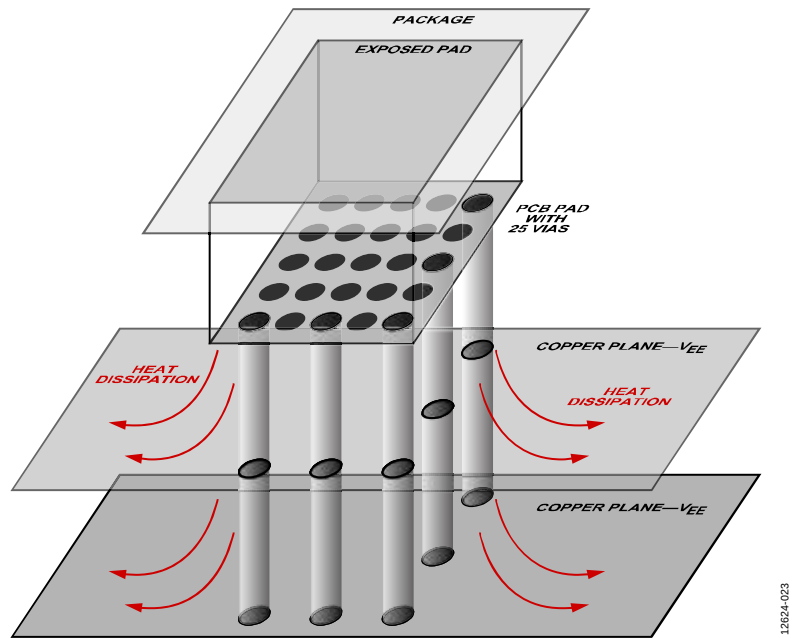
Figure 23. Connecting Vias to VEE
