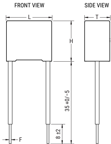
Insulated Rigid Leads
