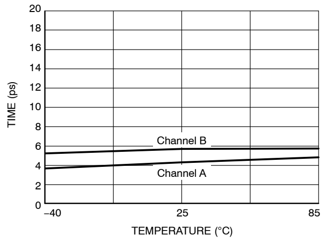
Figure 4. Within-Device Skew vs. Temperature at V_{CC} = 3.3\text{ V}
