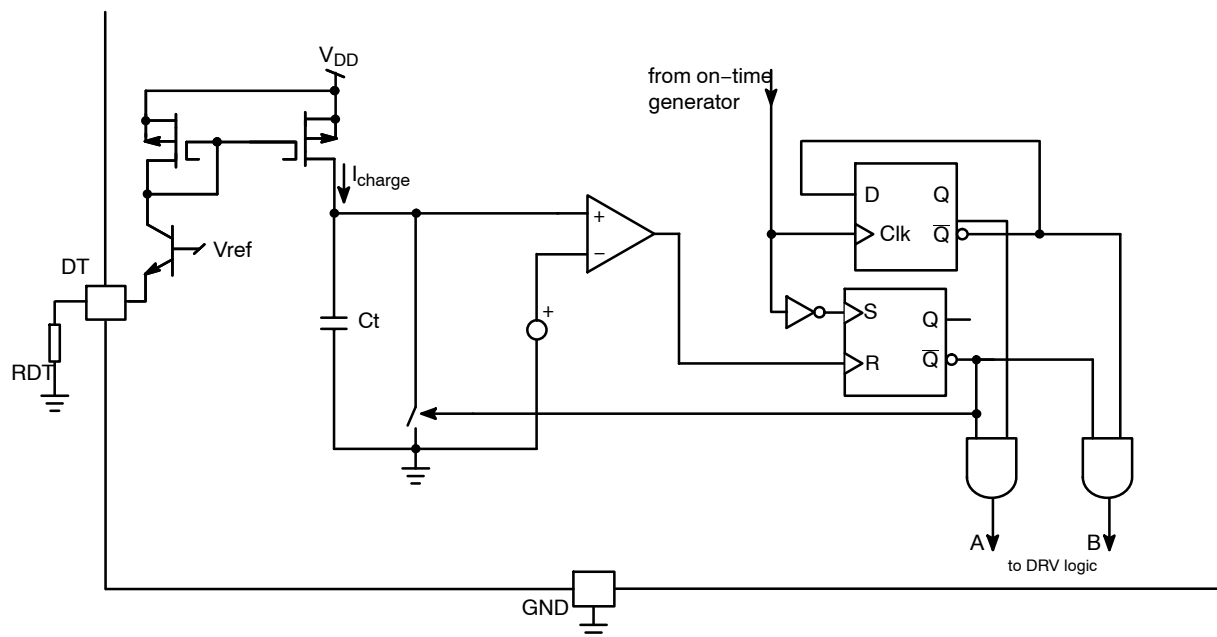
Figure 32. Dead-Time Generation
